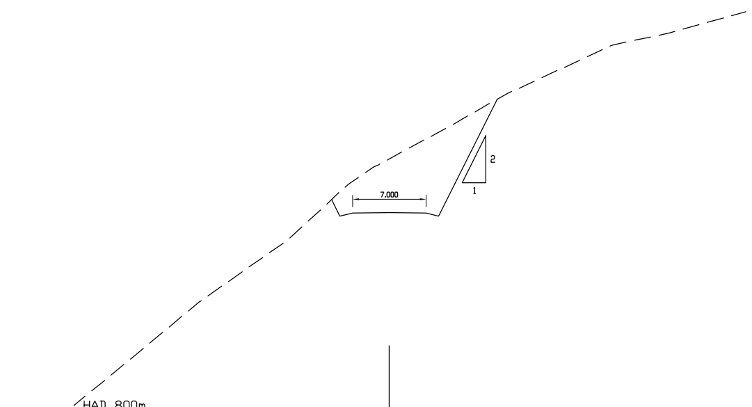
SECTION G SCALE 1:250(A1) 86
