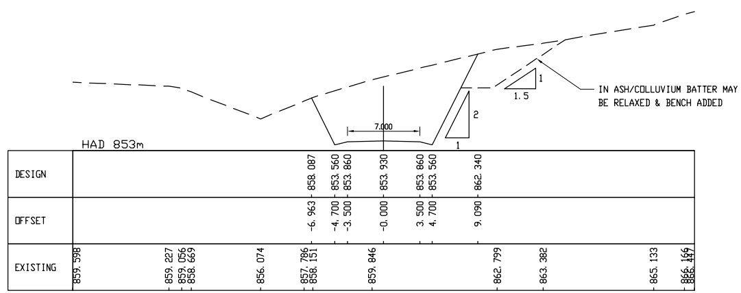
SECTION G SCALE 1:250(A1) 86
