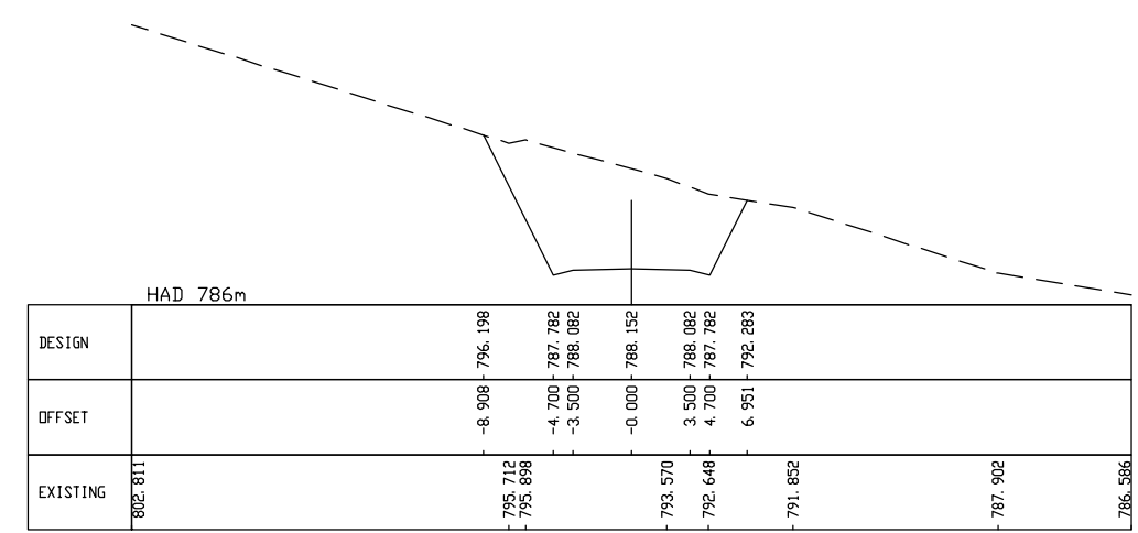
SECTION J SCALE 1:250(A1) 87
